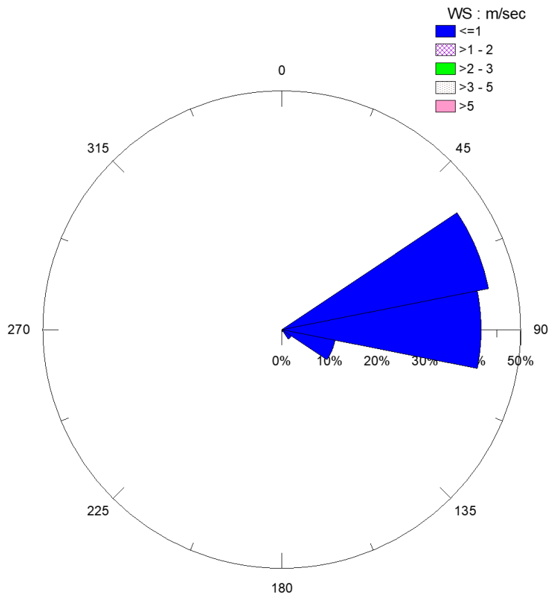
110/12/17~111/1/14 Wind Chart
