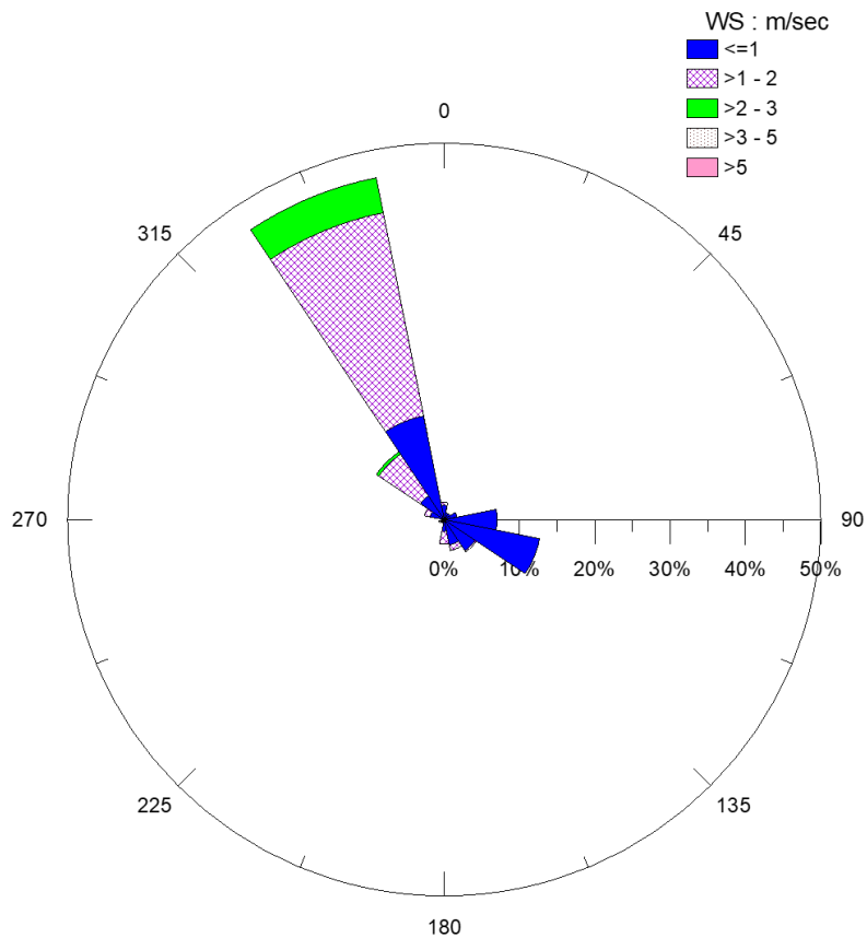
113/11/27~113/12/19 Wind Chart
