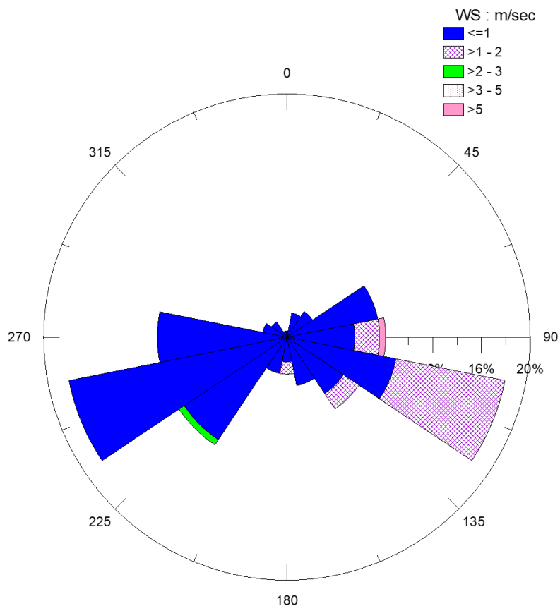
11/20~11/30 Wind Chart
