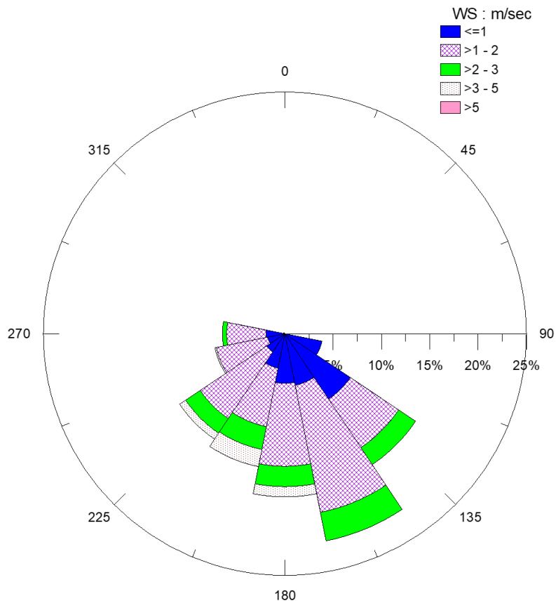
112/9/27~112/10/25 Wind Chart
